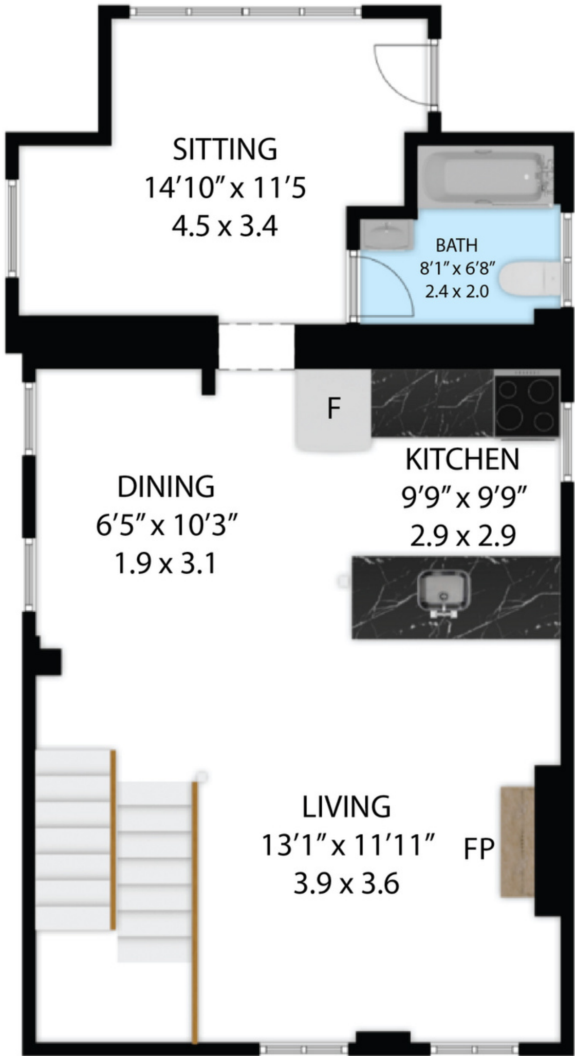
MAIN FLOOR
