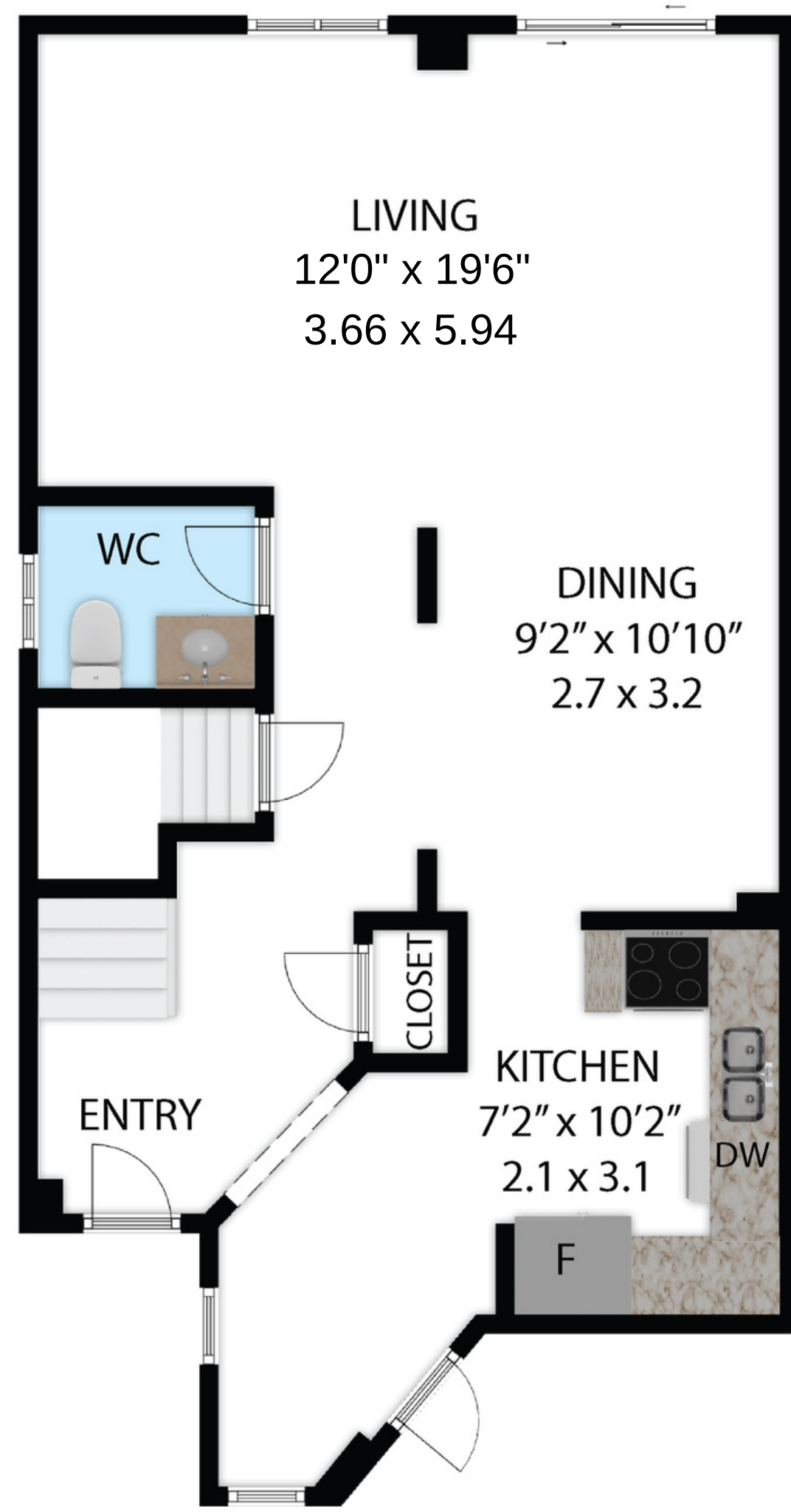
MAIN FLOOR
