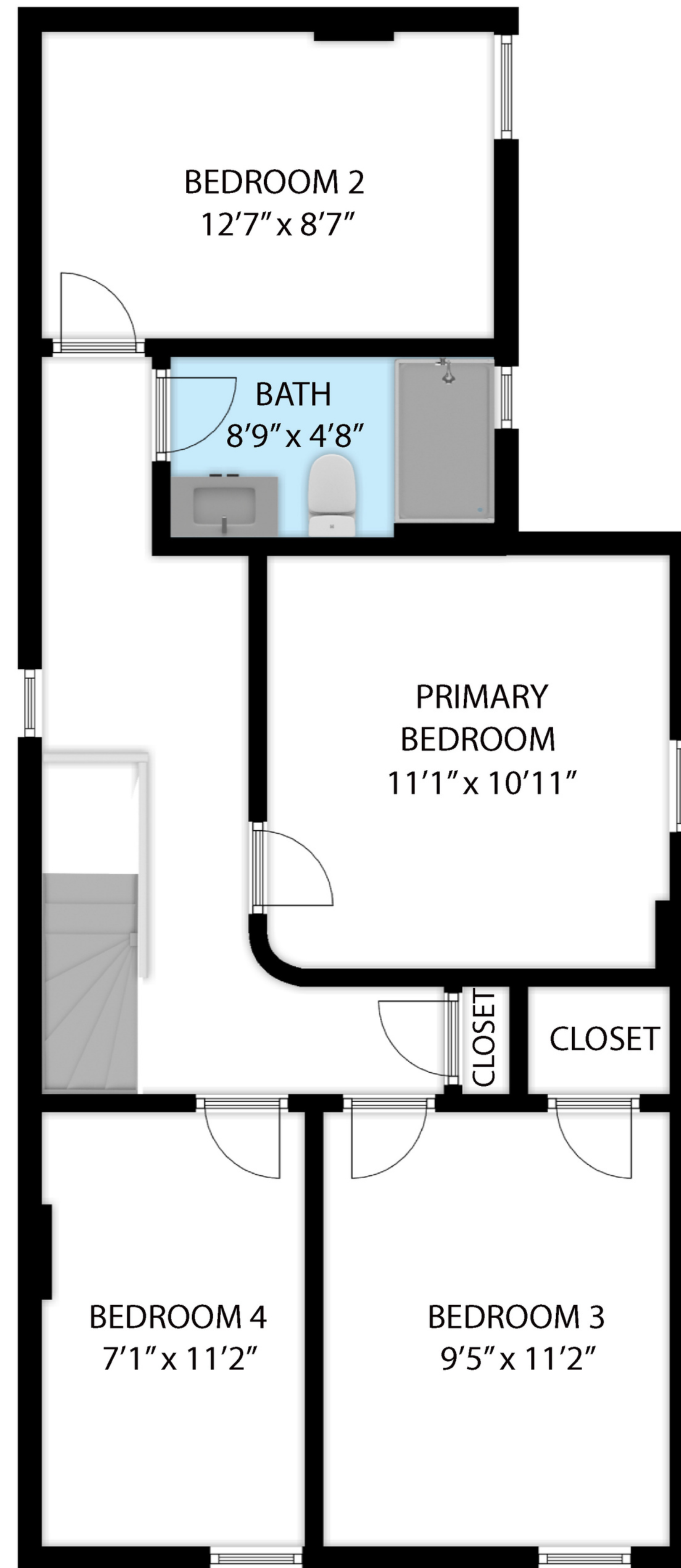
SECOND FLOOR
